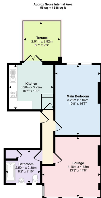
Floorplan
